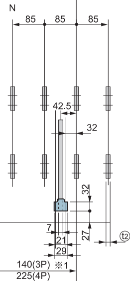
Terminal Vertical
